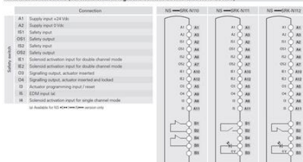
Internal connections (versions with integrated control device unit for 1 device)
