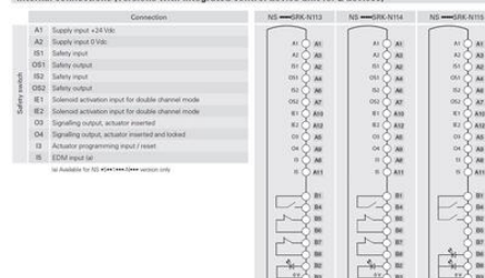
Internal connections (versions with integrated control device unit for 2 devices)
