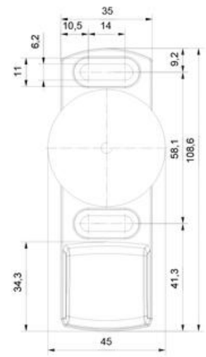
Anchor plate
