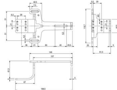
Internal fixing plate (articles AN G••••••••)
