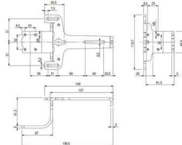
Internal fixing plate (articles AN S•••••)
