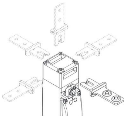
Switch FY 6-D1D- Operating principle D, with sealable auxiliary release device
