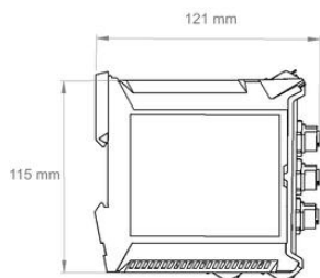
DCS-103E — Dimensions
