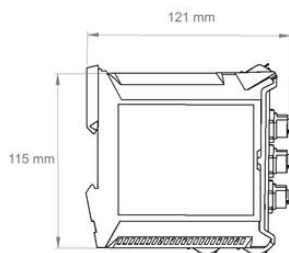
DCS-103E — Dimensions
