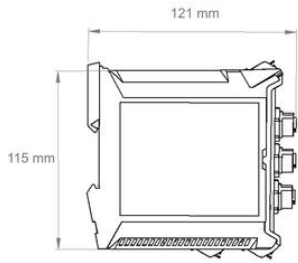
DCS-103E - Dimensions
