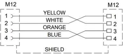
WIRING DIAGRAM
