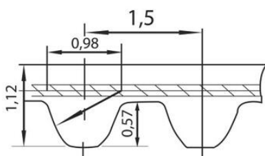
Kuggrem S1,5M
