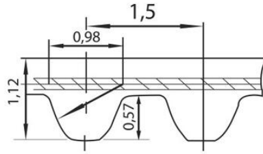
Kuggrem S1,5M
