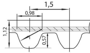
Kuggrem S1,5M
