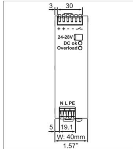
Fig. 22-1 Front view
