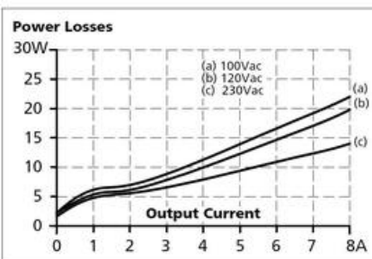
Fig. 9-2 Losses vs. output current at 36V, typ.
