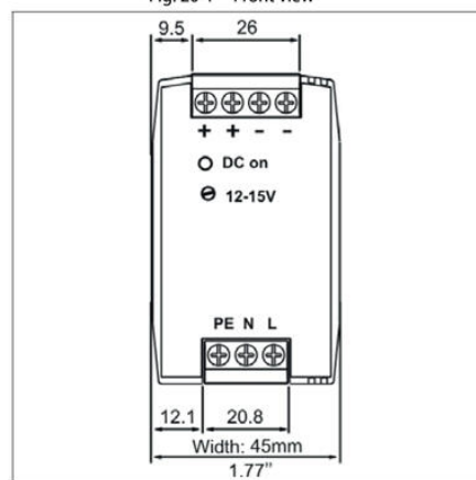
Fig. 20-1 Front view
