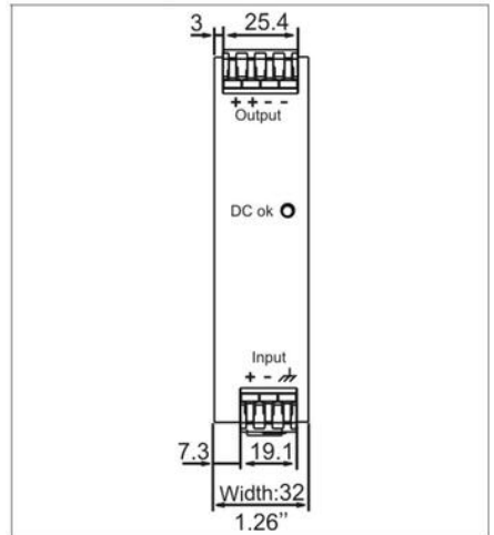
Fig. 19-1 Front view
