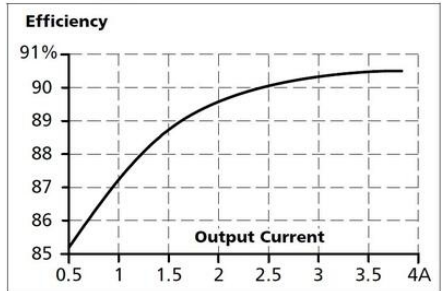
Fig. 7-1 Efficiency vs. output current at 24V, typ.
