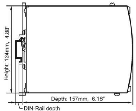
Fig. 22-2 Side view
