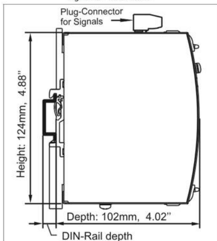
Fig. 21-2 Side view
