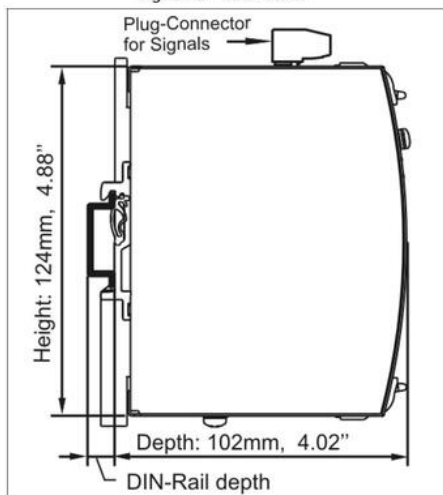
Fig. 21-2 Side view
