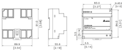
CHROME Chrome DIN Rail Power Supply 12V 100W 1 Phase / DRC-12V100W1AZ
