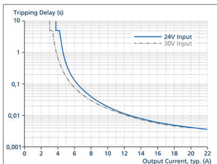
CH3 to CH8 tripping diagrams in Fast mode
