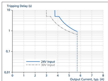
CH1 and CH2 tripping diagrams in Slow mode
