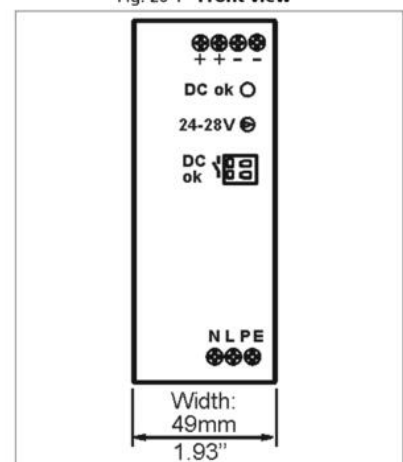
Fig. 20-1 Front view
