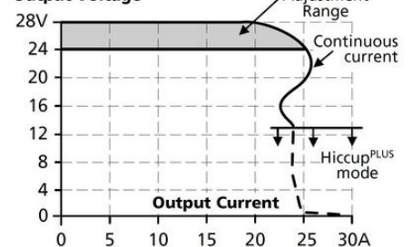
Output Voltage
