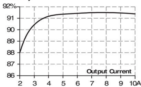
Efficiency
