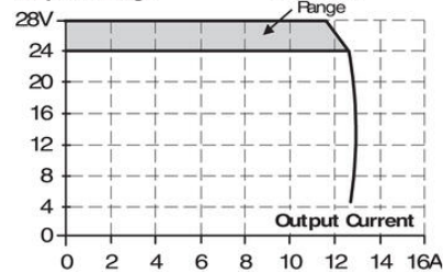
Output Voltage
