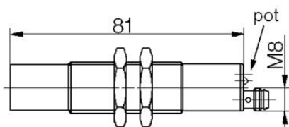
NPN - Proximity Switch
