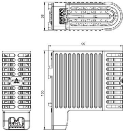
Heater LTS 064
