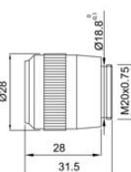
22mm LENS
