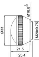
40mm LENS
