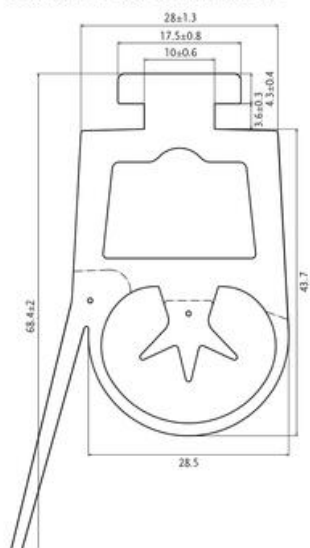
Profile cross-section Contact-Duo 3100.0804B
