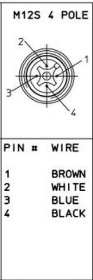
Mating face view:
