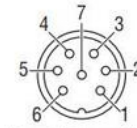
Front side molded 7P Female connector
