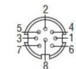
Front side Molded OEM connector 8p M16 male
