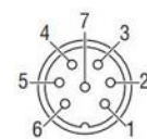
Front side molded 7P Female connector
