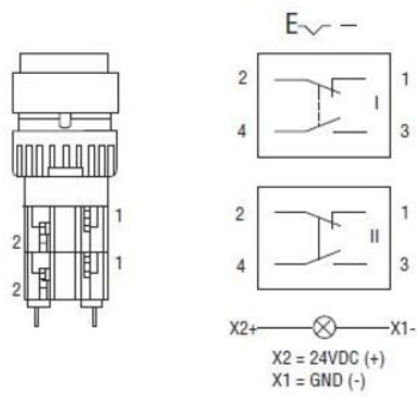
Wiring diagram
