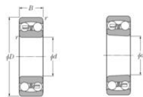
Cylindrical bore
