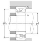
Cylindrical bore
