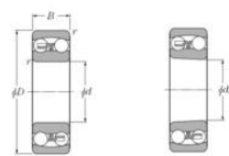
Cylindrical bore
