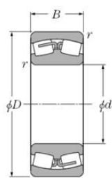
Cylindrical bore
