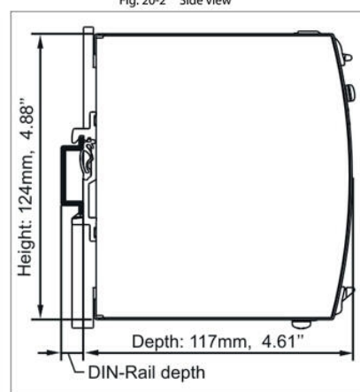
Fig. 20-2 Side view
