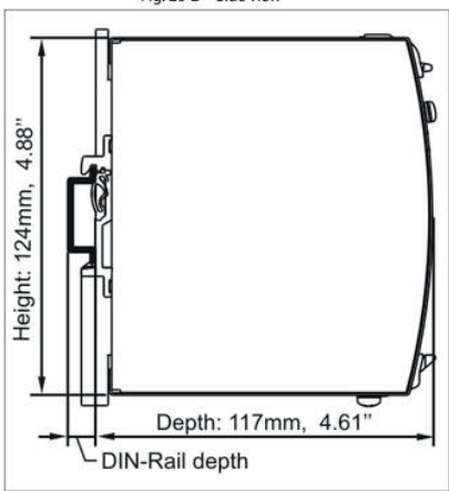
Fig. 20-2 Side view
