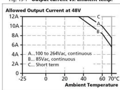
Fig. 15-1 Output current vs. ambient temp.
