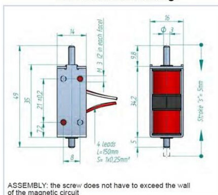
Dimensional drawing:
