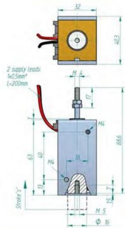
Locked solenoid
