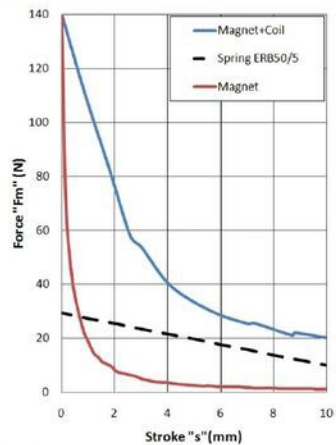
Force-Stroke Curve (F-S)
