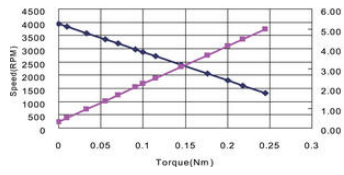
MB054TP100 CURVE
