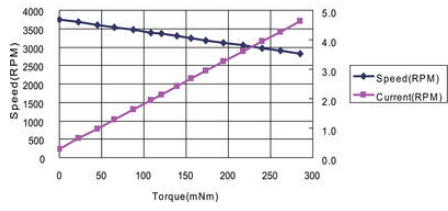
MB063KG100 CURVE
