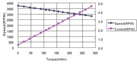
MB063G100 CURVE
