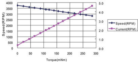
MB063KG100 CURVE
