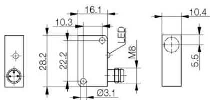
PNP – Proximity Switch
