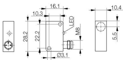
PNP – Proximity Switch
