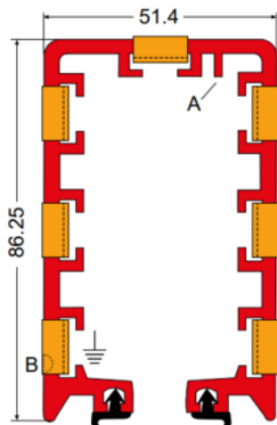
Housing RC7 with AS7
