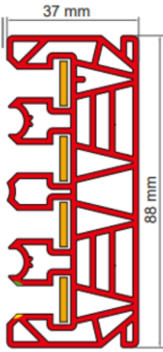
Housing PR4 with copper conductors
