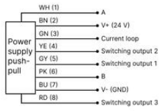
Pinout diagram sensor
