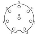
M12 9-pin a-coded male layout
