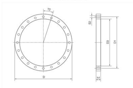
iglidur® PRT spacer ring heavy duty, steel
