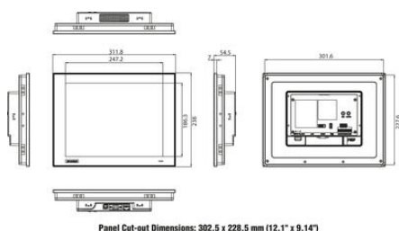
Panel Cut-out Dimensions: 302.5 x 228.5 mm (12.1\" x 9.14\")
