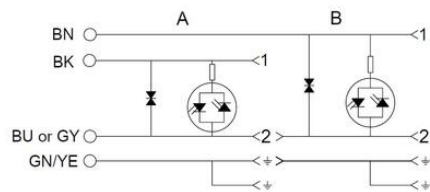
ELECTRICAL DIAGRAM - S0
