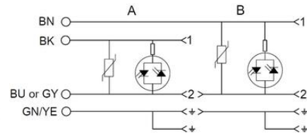
ELECTRICAL DIAGRAM - C4
