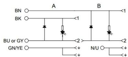
ELECTRICAL DIAGRAM - C3
